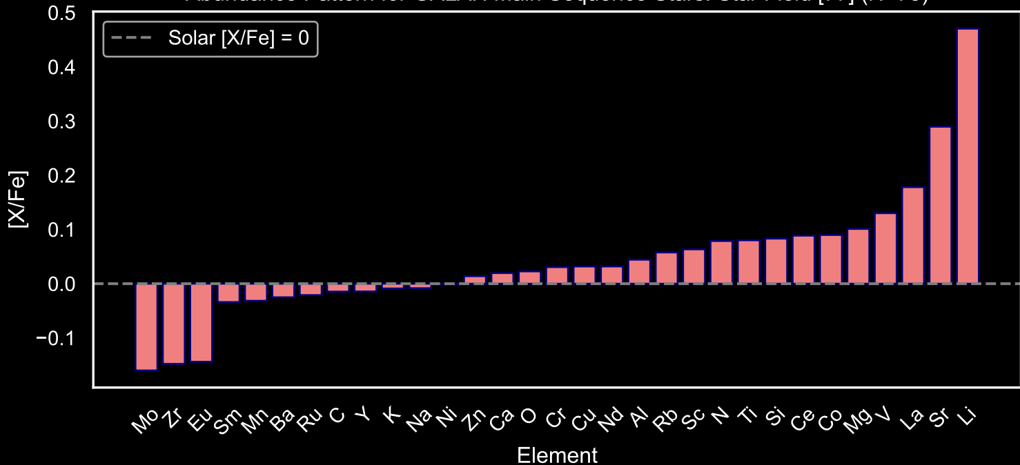
Abundance Pattern for GALAH Main Sequence Stars: Star Field [77] (N=75)
