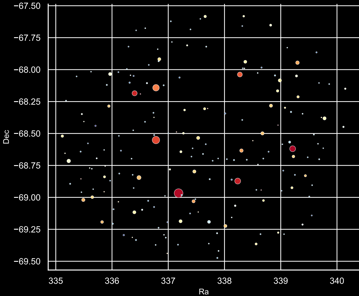
Field [77] Ra [337.49] Dec [-68.58] Stars: 183
