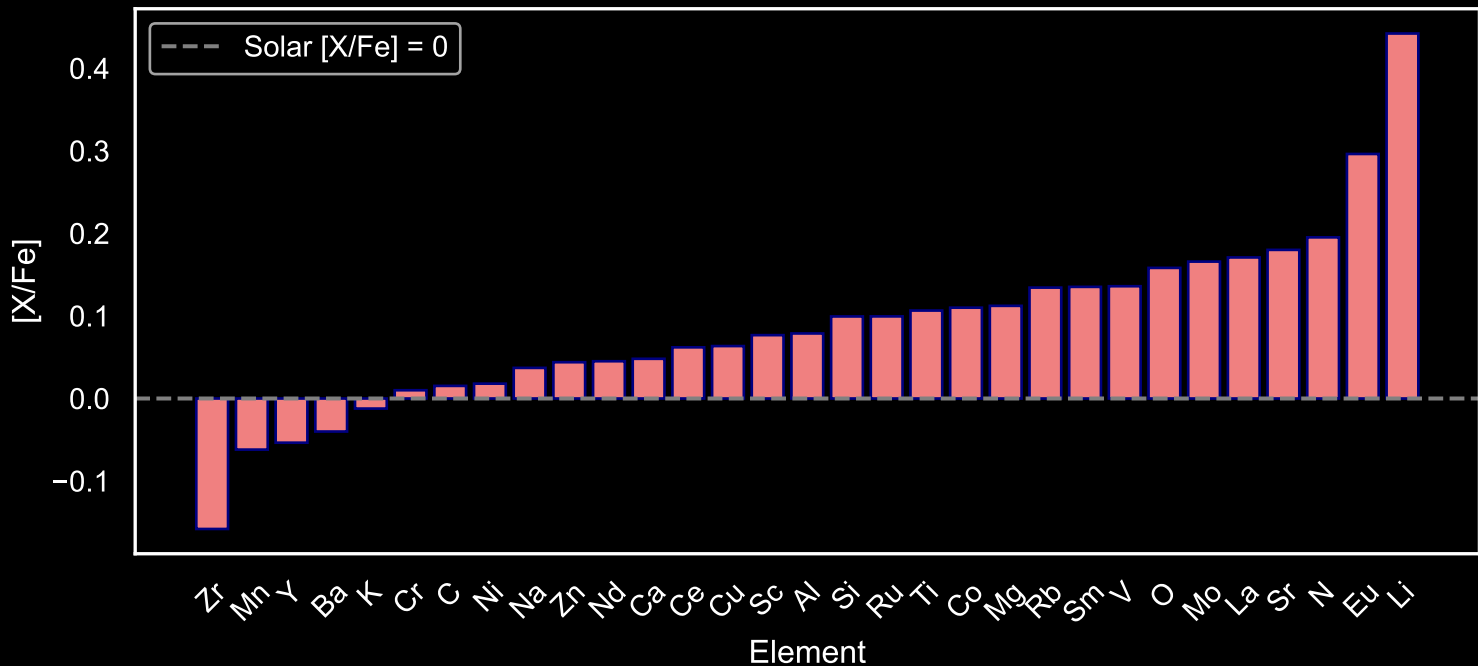
Abundance Pattern for GALAH Star Field [77] (N=183)
