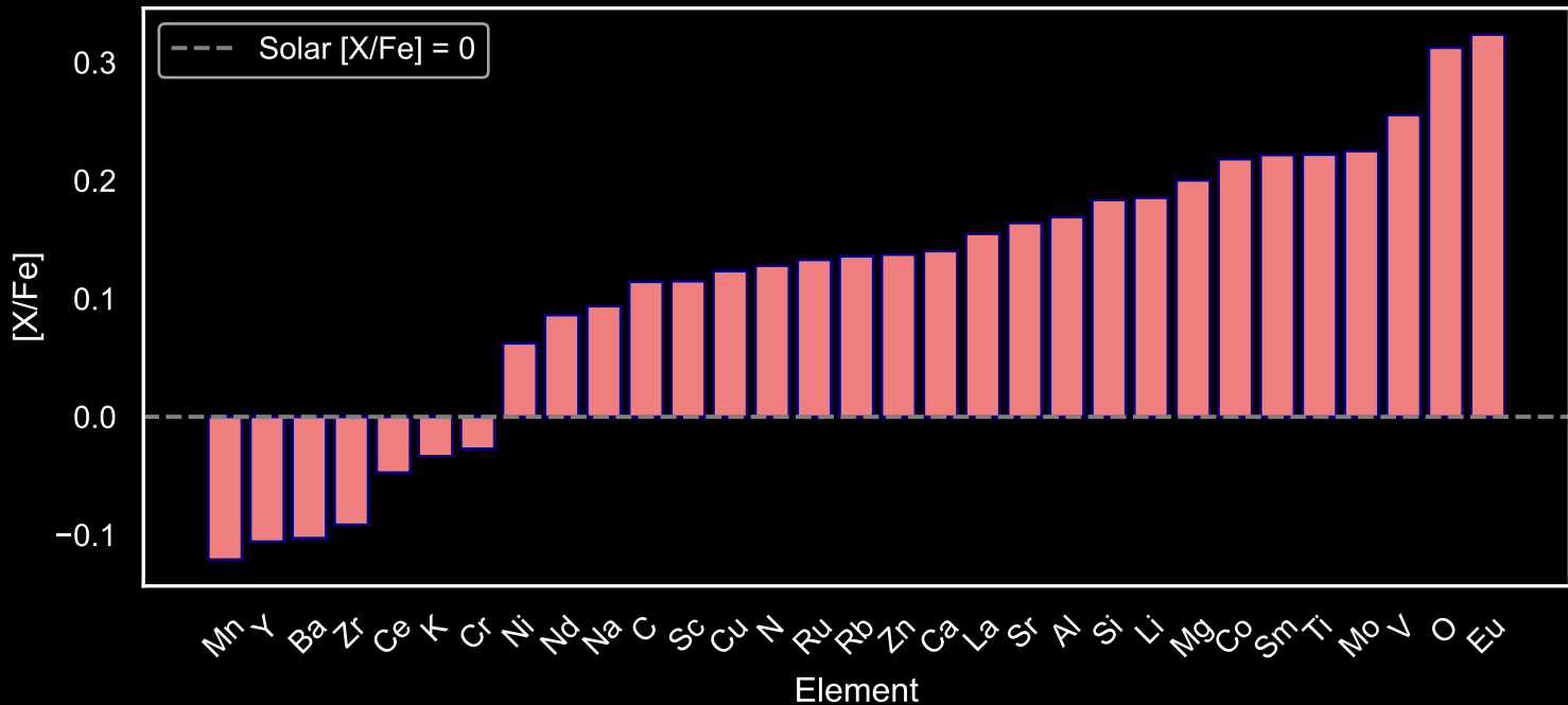
Abundance Pattern for GALAH Red Giants: Star Field [77] (N=48)
