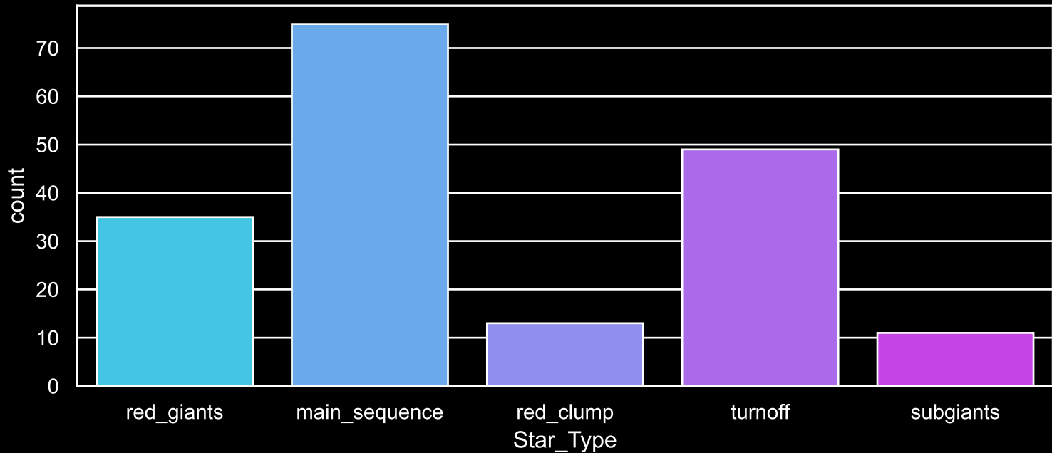
Field [77] Count plot of Star Type
